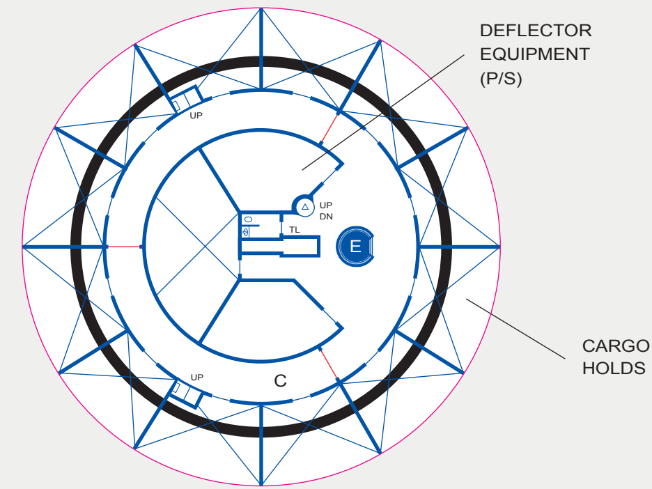
DECK 10: DEFLECTOR EQUIPMENT / CARGO
