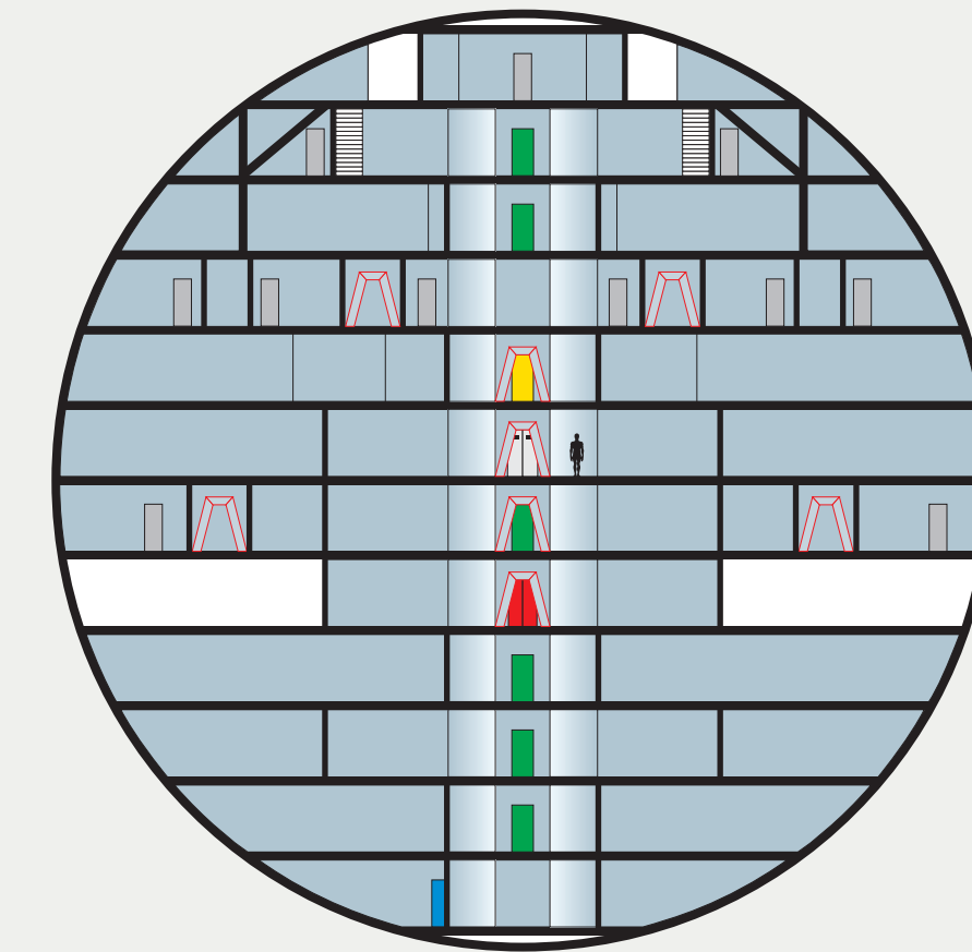
CROSS-SECTION A-A
