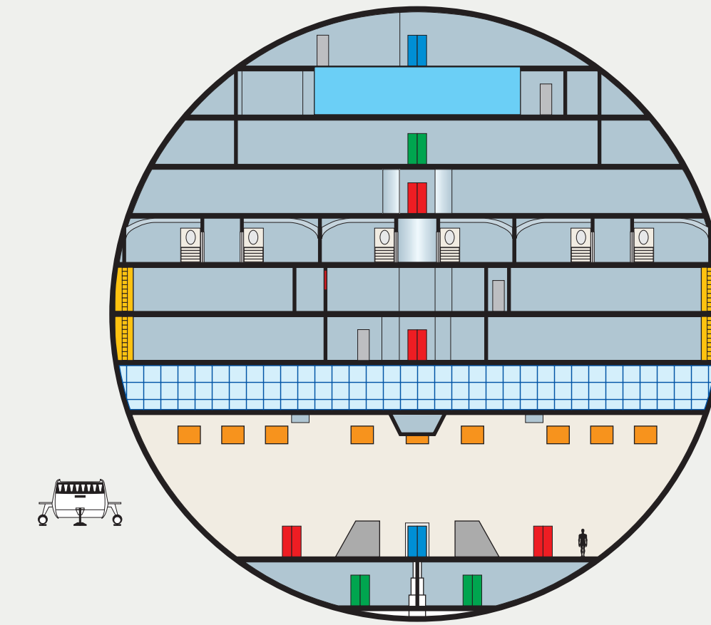
CROSS-SECTION F-F
