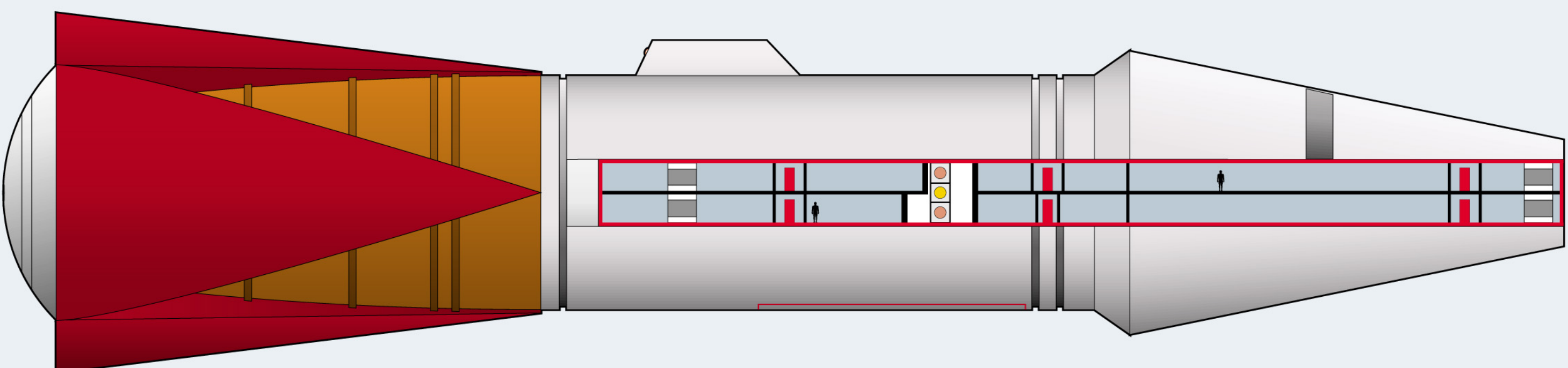
STARBOARD VIEW ALONG THE SEPARATION PLANE OF THE PORT ENGINE
