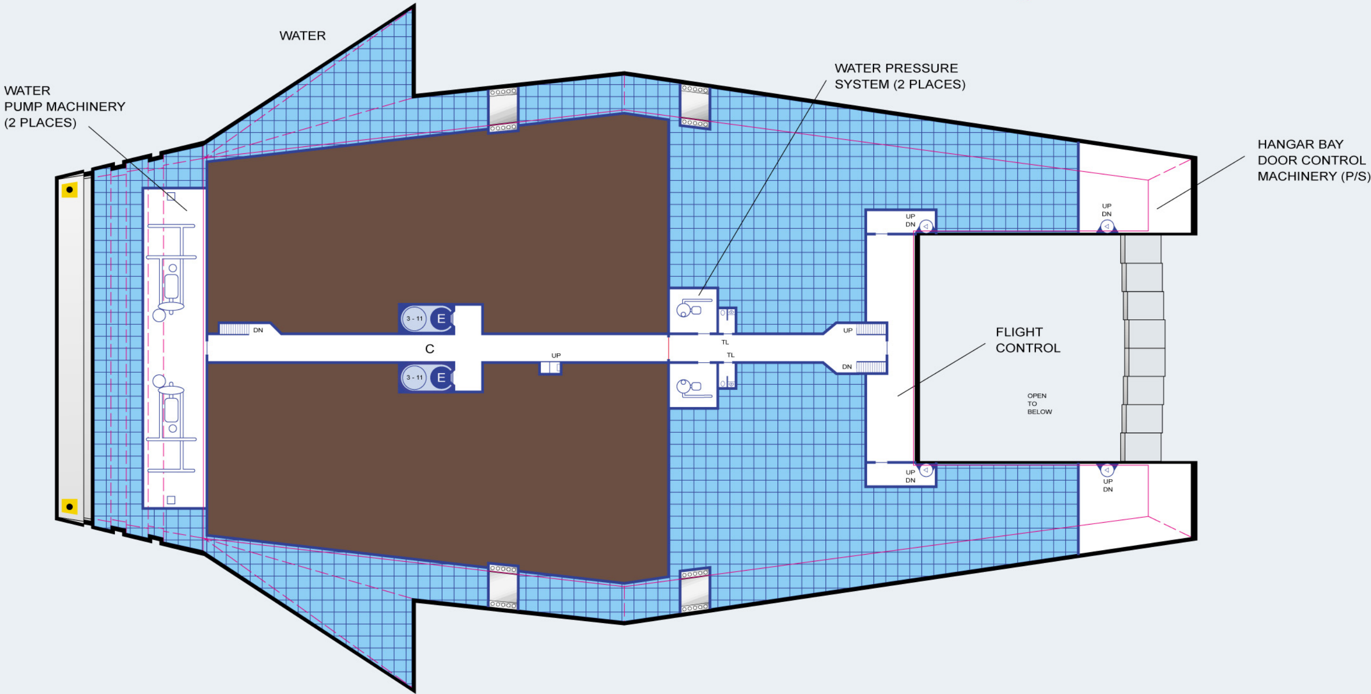
DECK 6: WATER / HANGAR BAY
