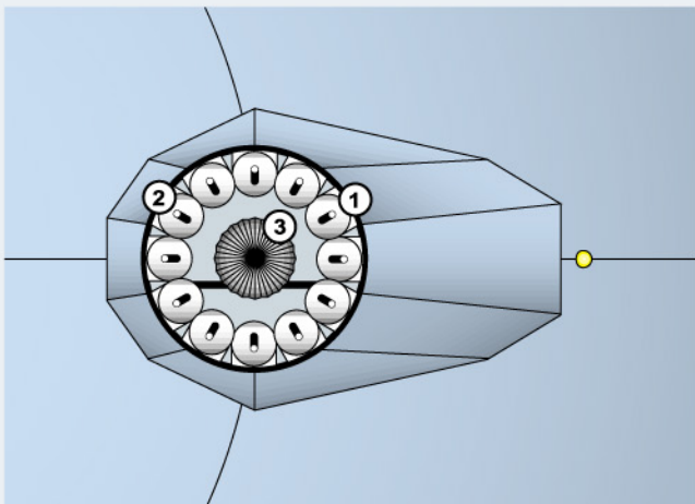
STARBOARD ENGINE SEPARATION PLANE (Cross-section)
