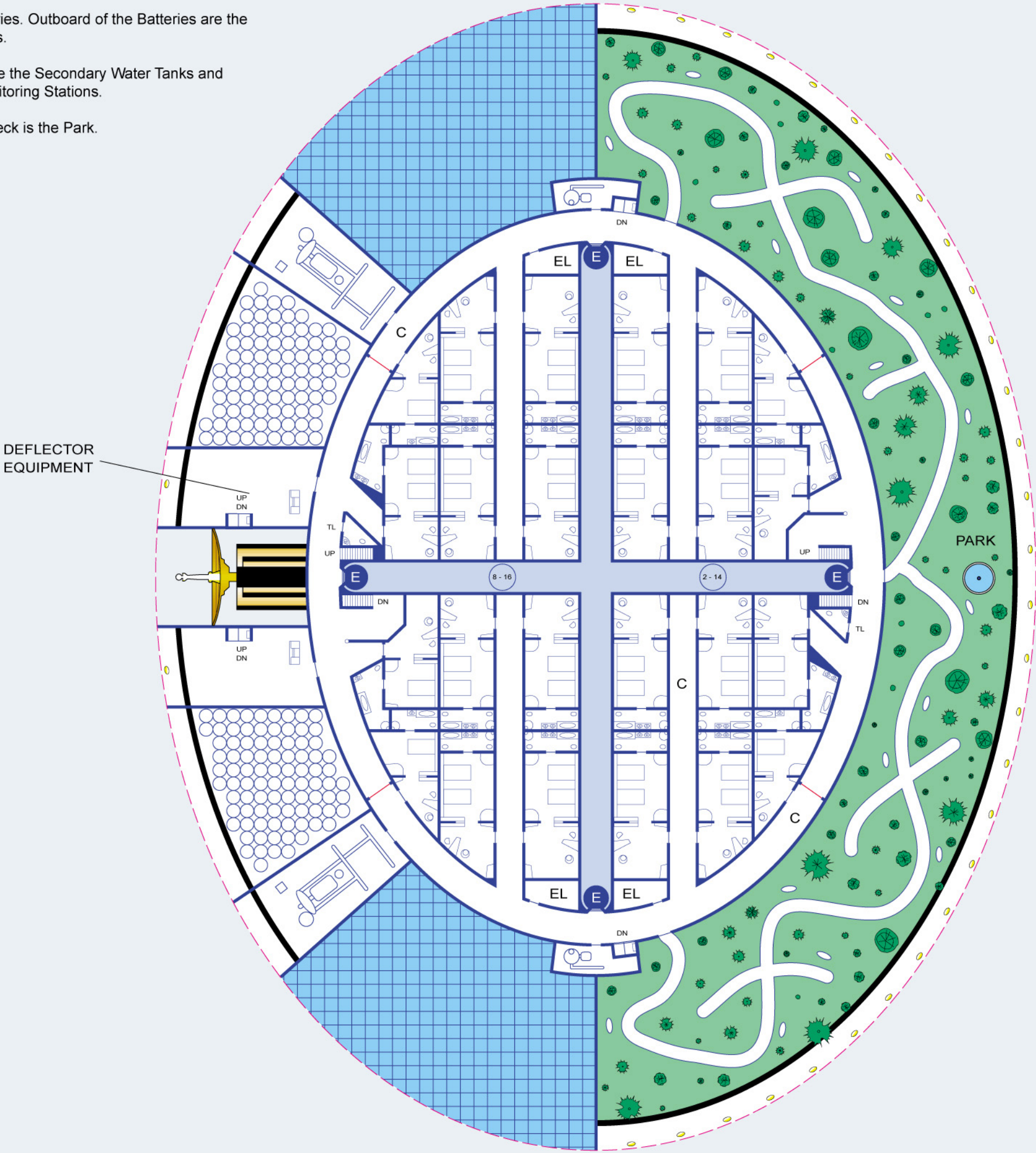
DECK 13: DEFLECTOR / WATER / PARK
