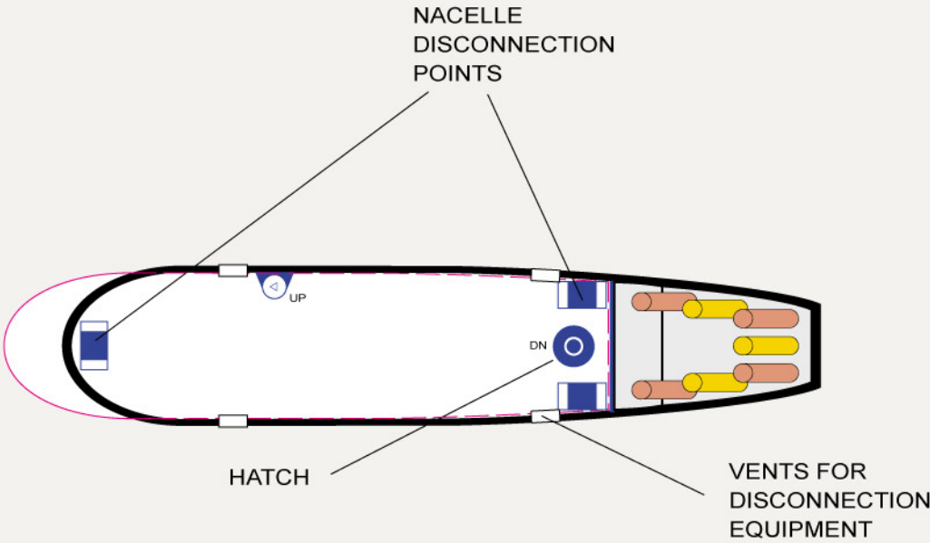
DECK 10: DORSAL
