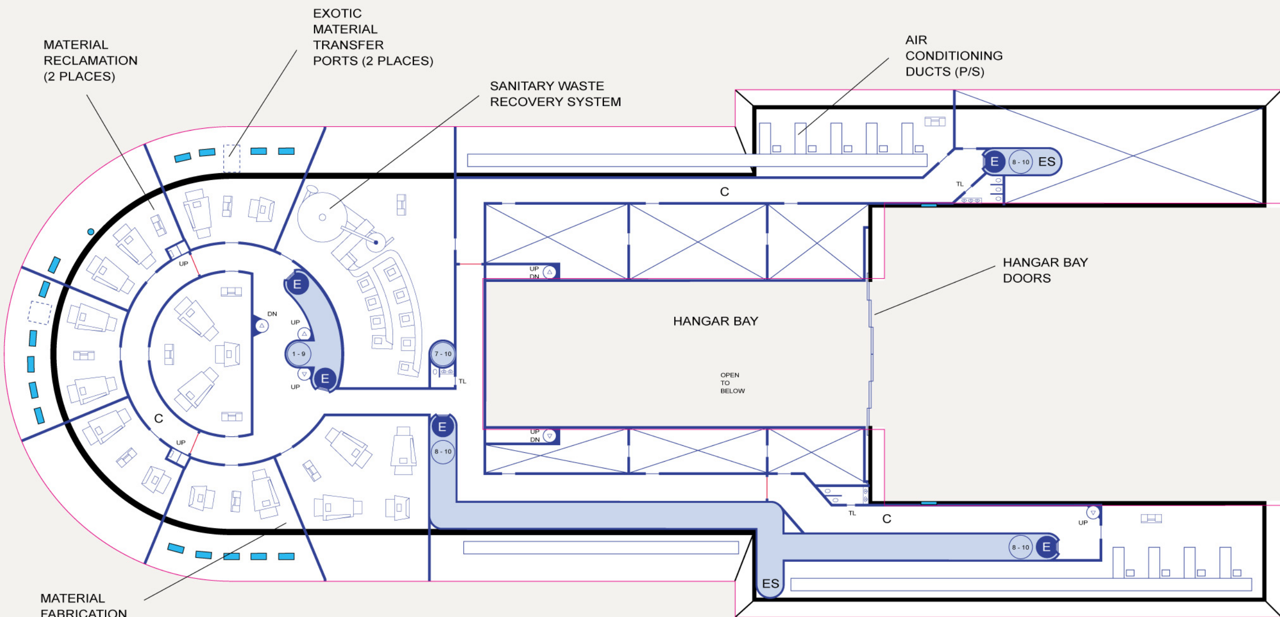
DECK 9: FABRICATION FACILITIES / HANGAR BAY
