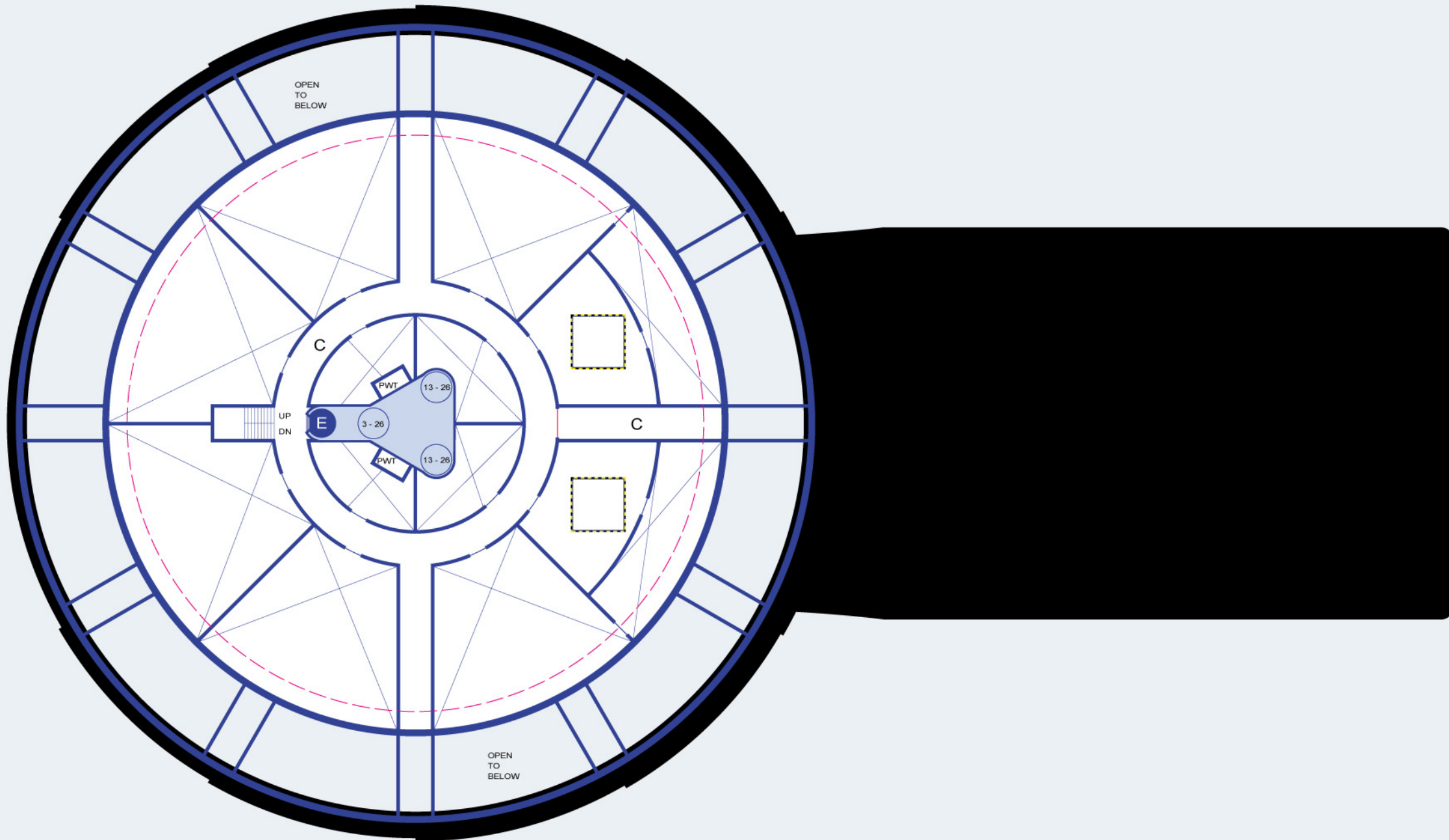
DECK 14: CLAMSHELL STRUCTURAL SUPPORT / CARGO
