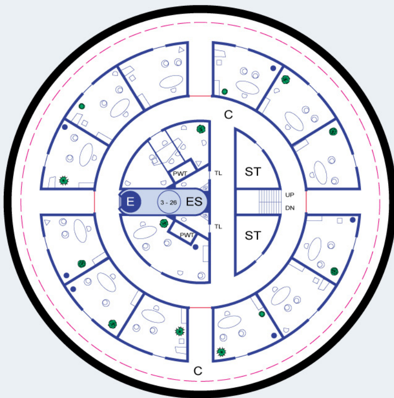
DECK 11: ADMINISTRATIVE OFFICES
