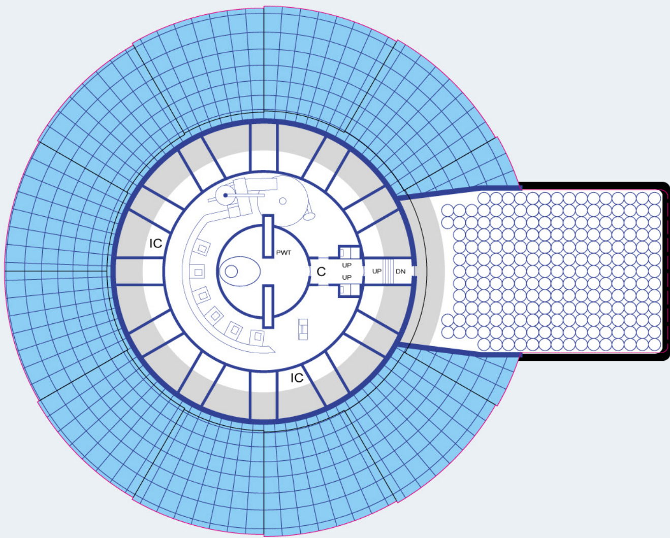
DECK 31G: FRESH WATER / SEWAGE TREATMENT / BATTERIES
