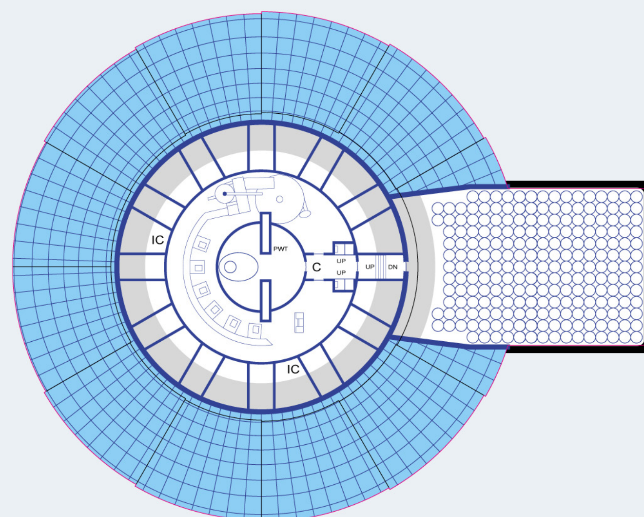
DECK 31Y: FRESH WATER / SEWAGE TREATMENT / BATTERIES
