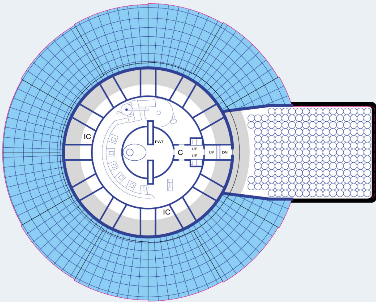
DECK 31R: FRESH WATER / SEWAGE TREATMENT / BATTERIES
