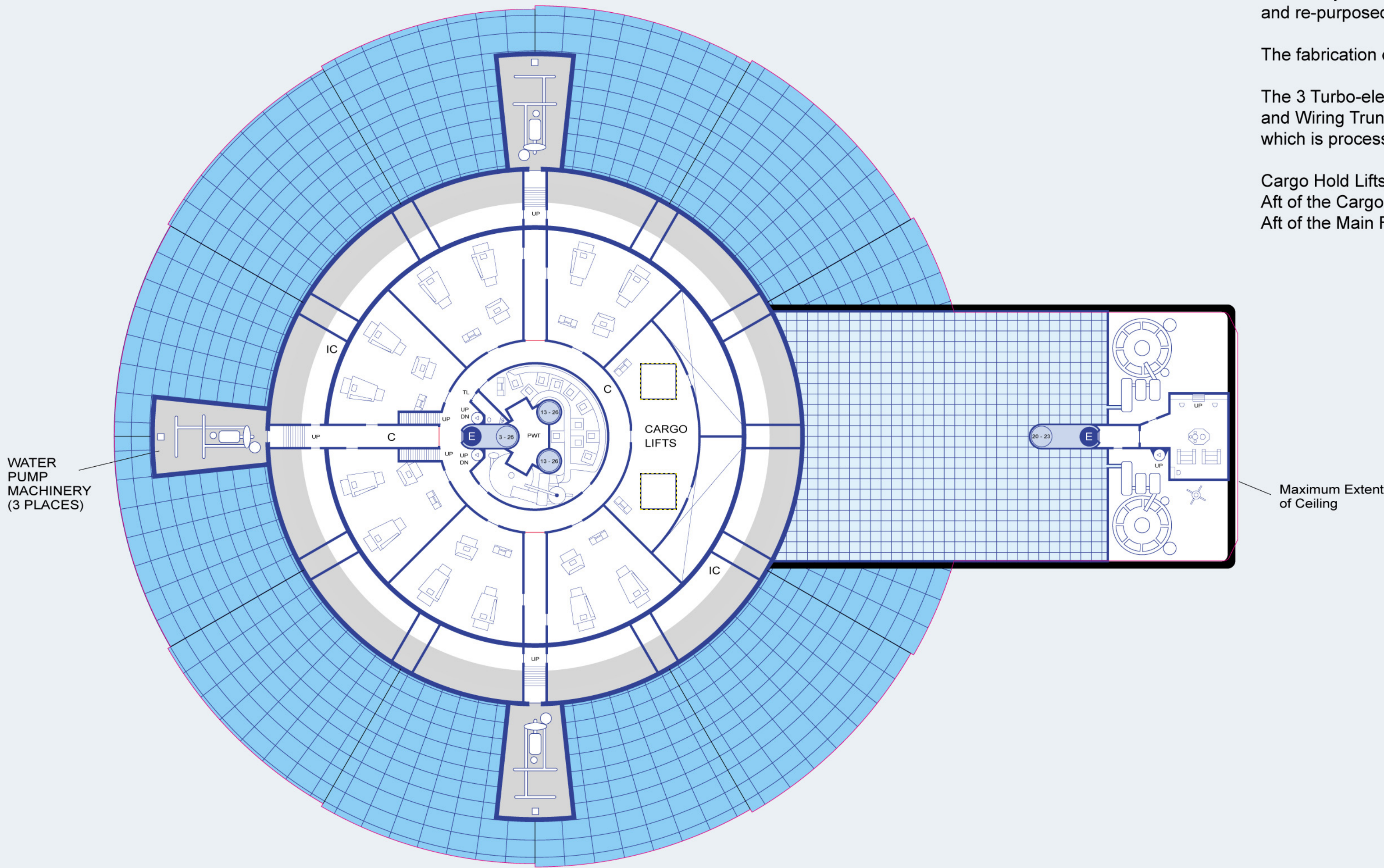
DECK 23: FRESH WATER / MATERIAL FABRICATION / FUEL / ENGINEERING
