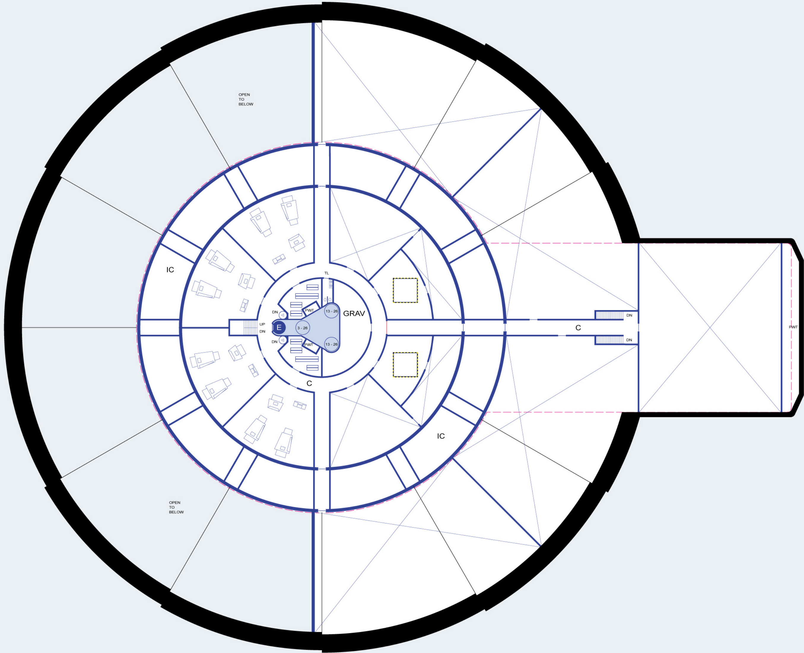
DECK 15: CLAMSHELL STRUCTURAL SUPPORT / CARGO
