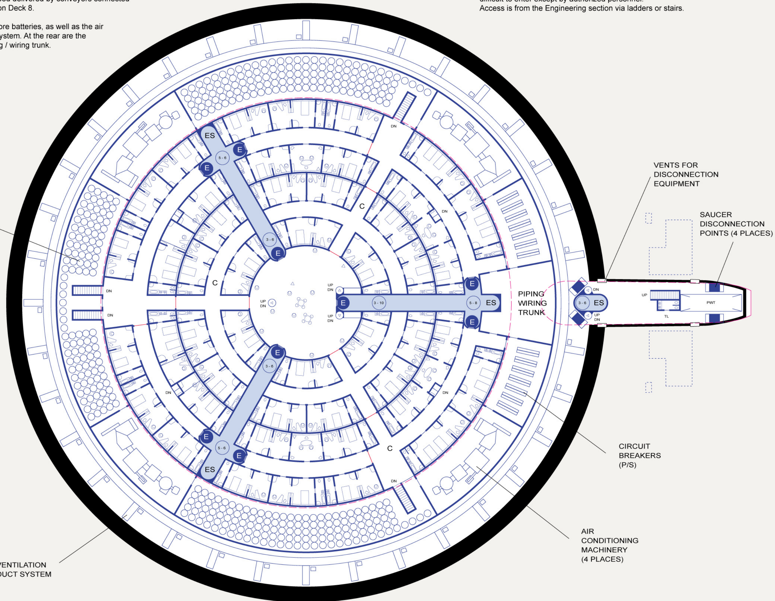
DECK 5: OFFICER'S QUARTERS
