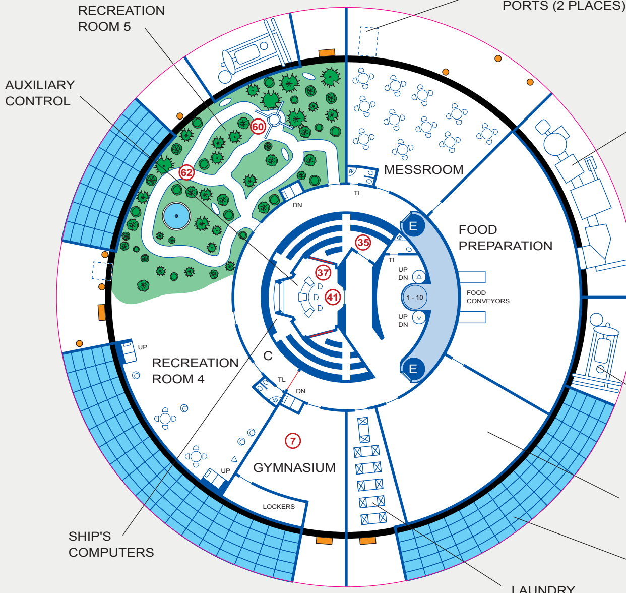
DECK 8: ENTERTAINMENT / RECREATION FACILITIES
