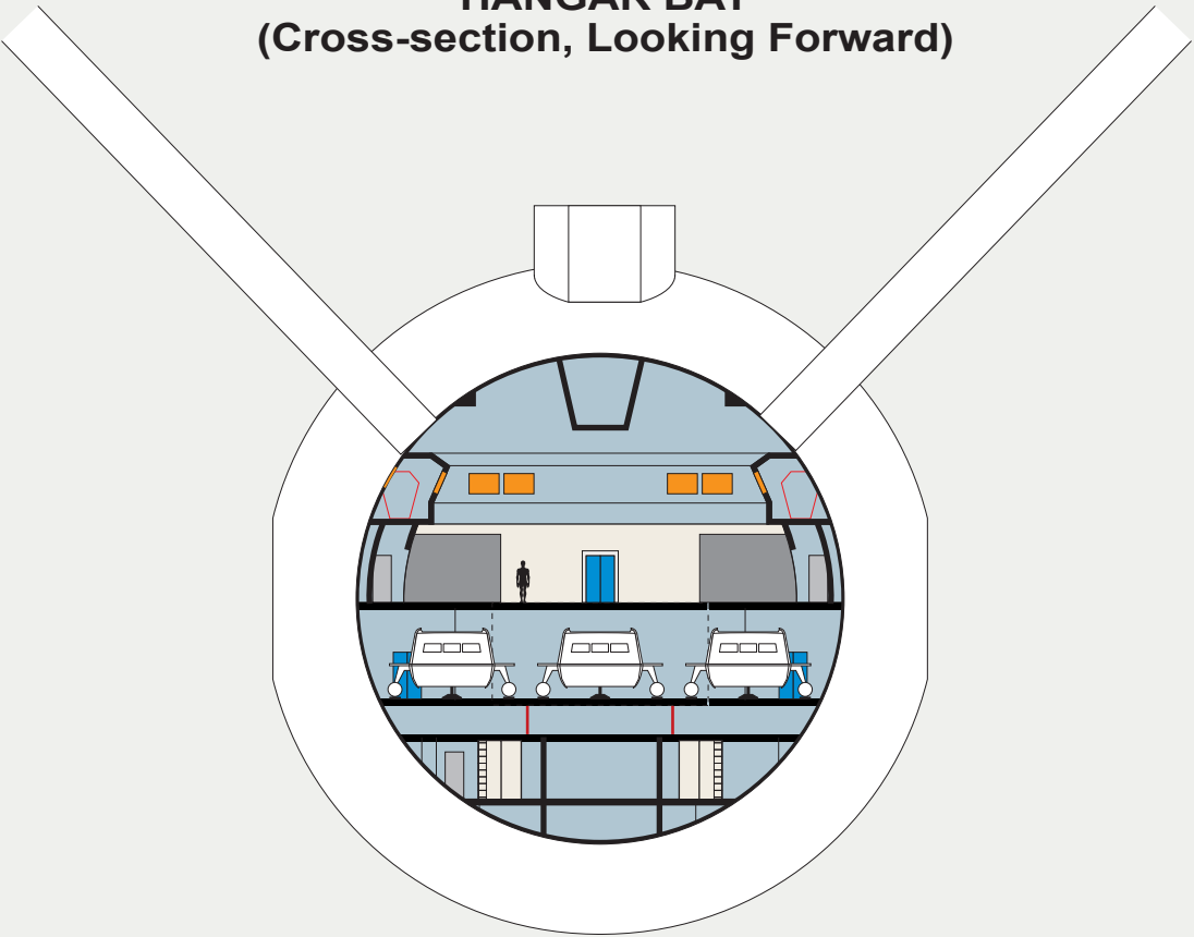
HEAVY CRUISER HANGAR BAY (Cross-section, Looking Forward)
