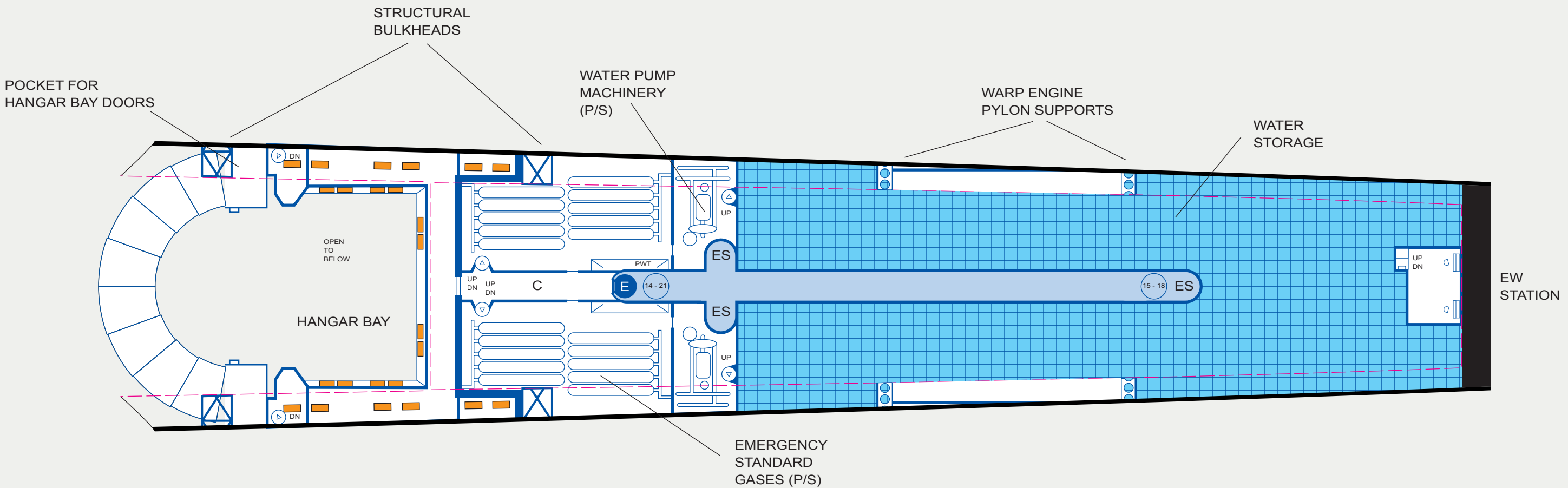
DECK 14: HANGAR BAY / STRONGBACK
