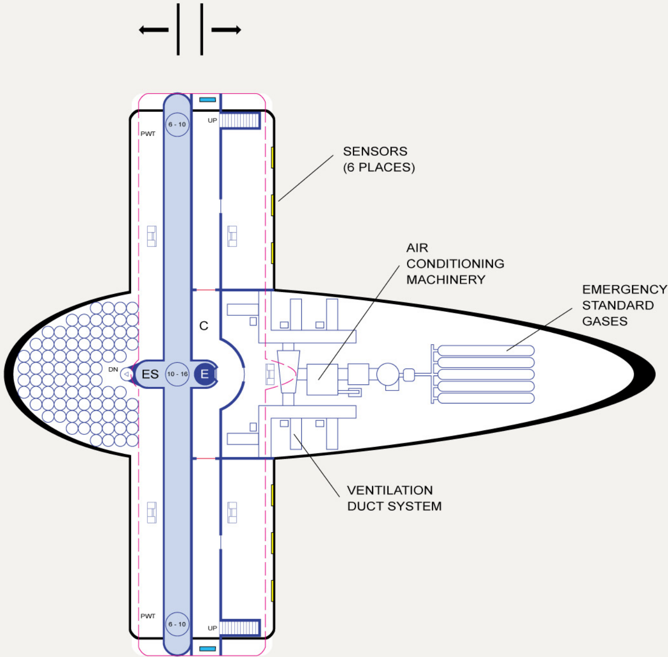
PYLONS (Cross-section, Fore and Aft)
