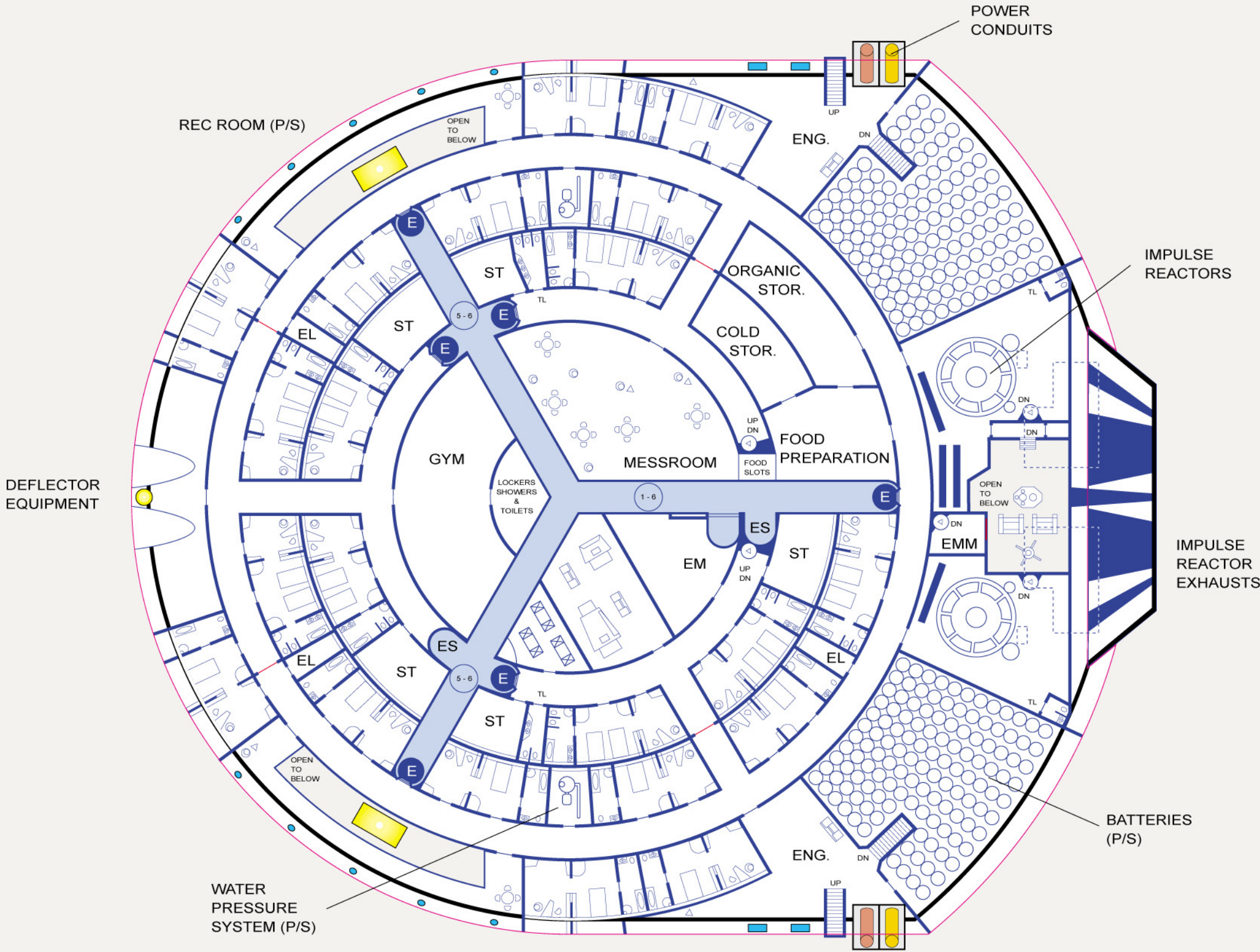
DECK 5: CREW QUARTERS / ENGINEERING
