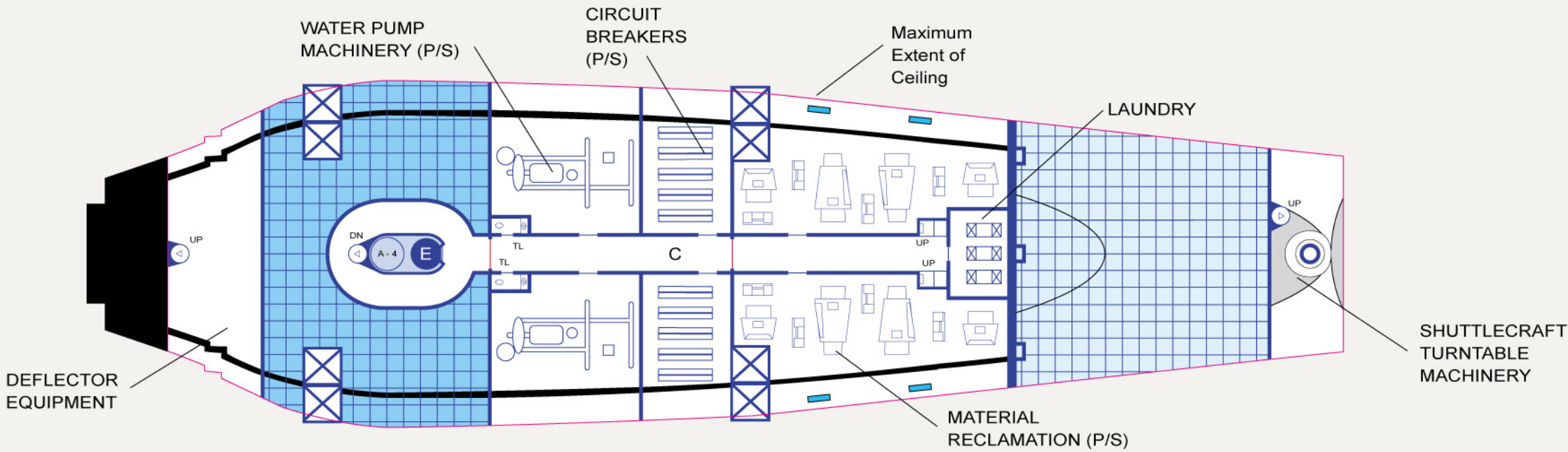
DECK I: ENVIRONMENTAL SERVICES
